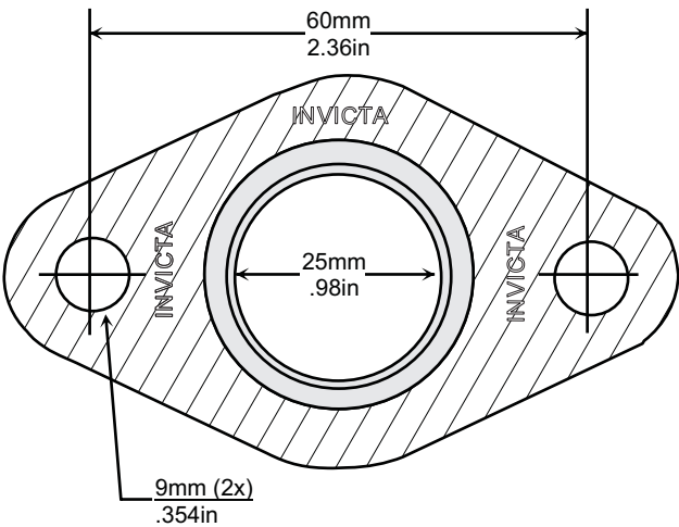
Single Layer Embossed Steel NOT TO SCALE
