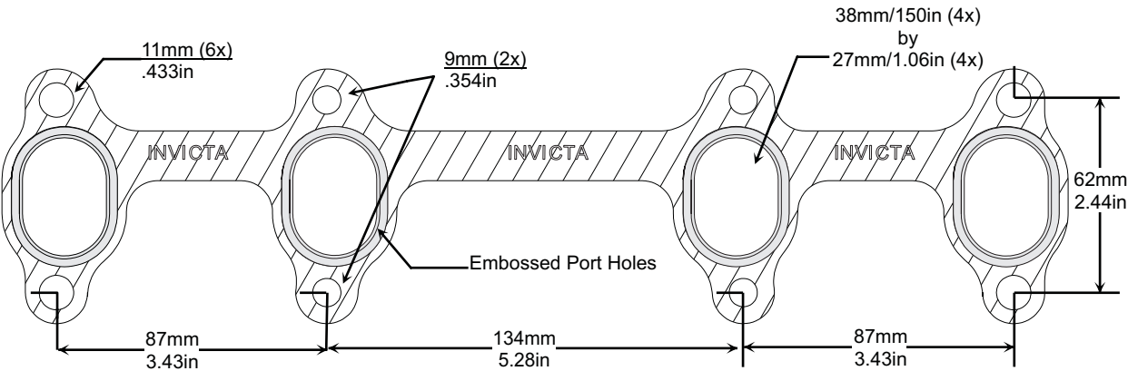
Single Layer Embossed Steel NOT TO SCALE
